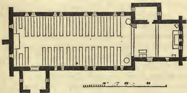
Ground plan of St. James' Church.
